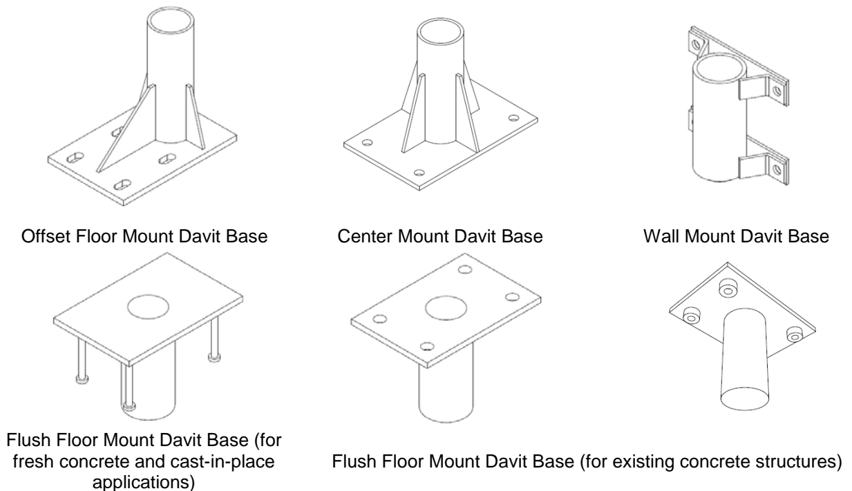
Figure 2.2: Pictorial Views of the Acceptable Davit Bases
