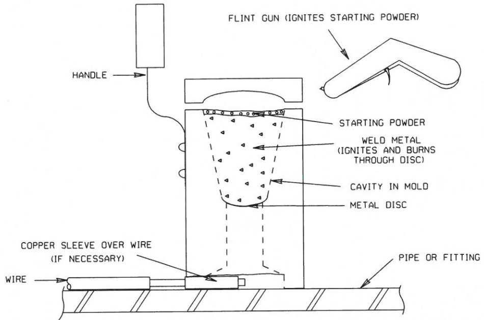
POSITIONING OF WIRE AND MOLD
