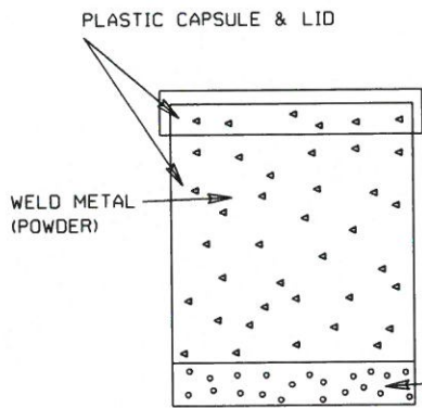
WELD METAL CAPSULE
