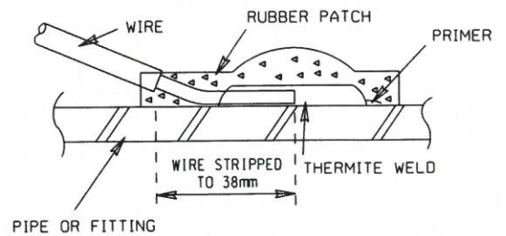
FINISHED WELD
