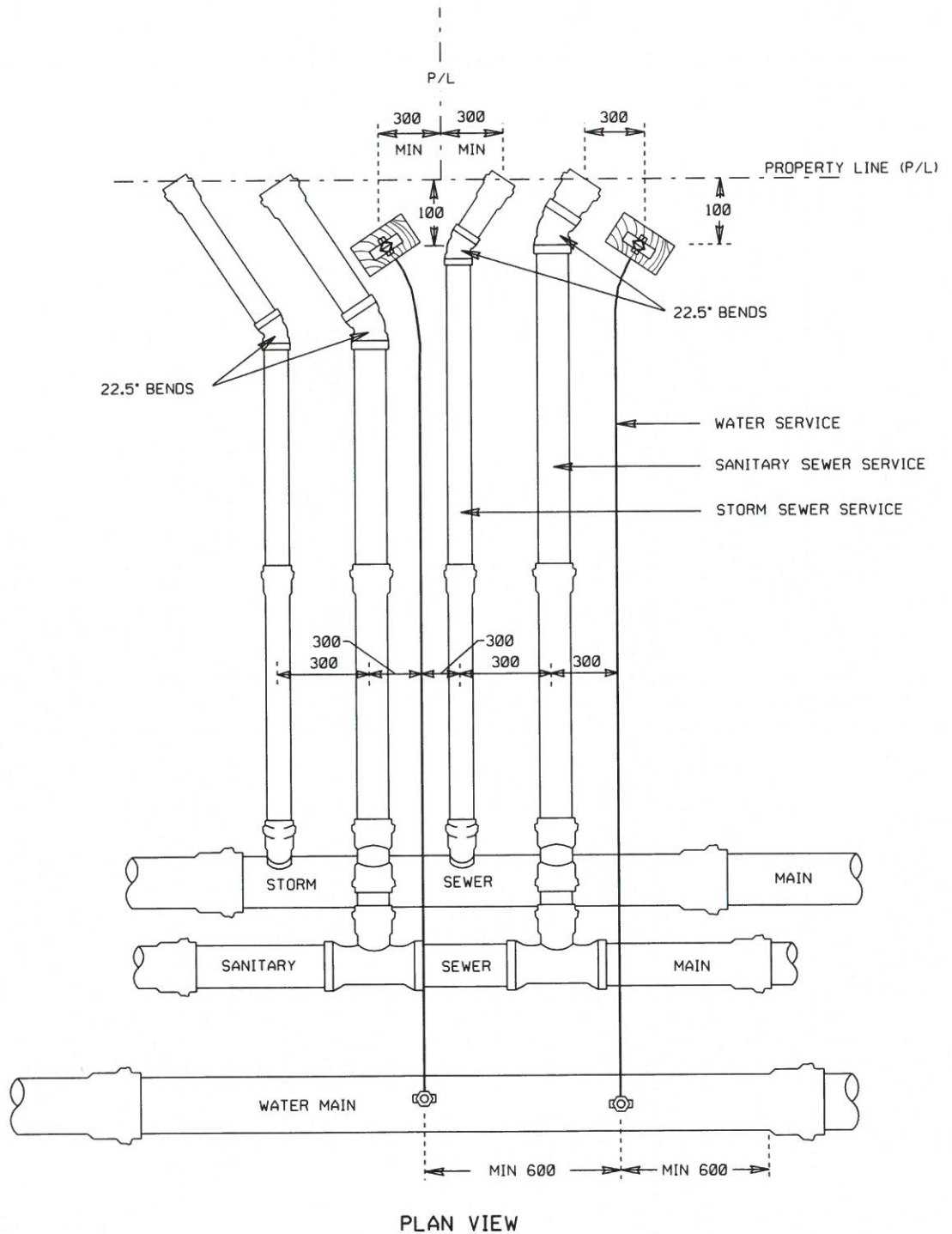
PLAN VIEW
