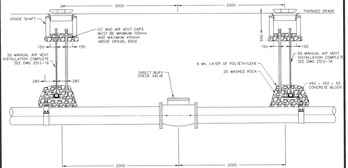
PROFILE
