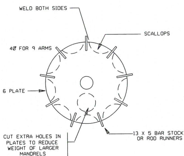
TRANSVERSE SECTION OF MANDREL
