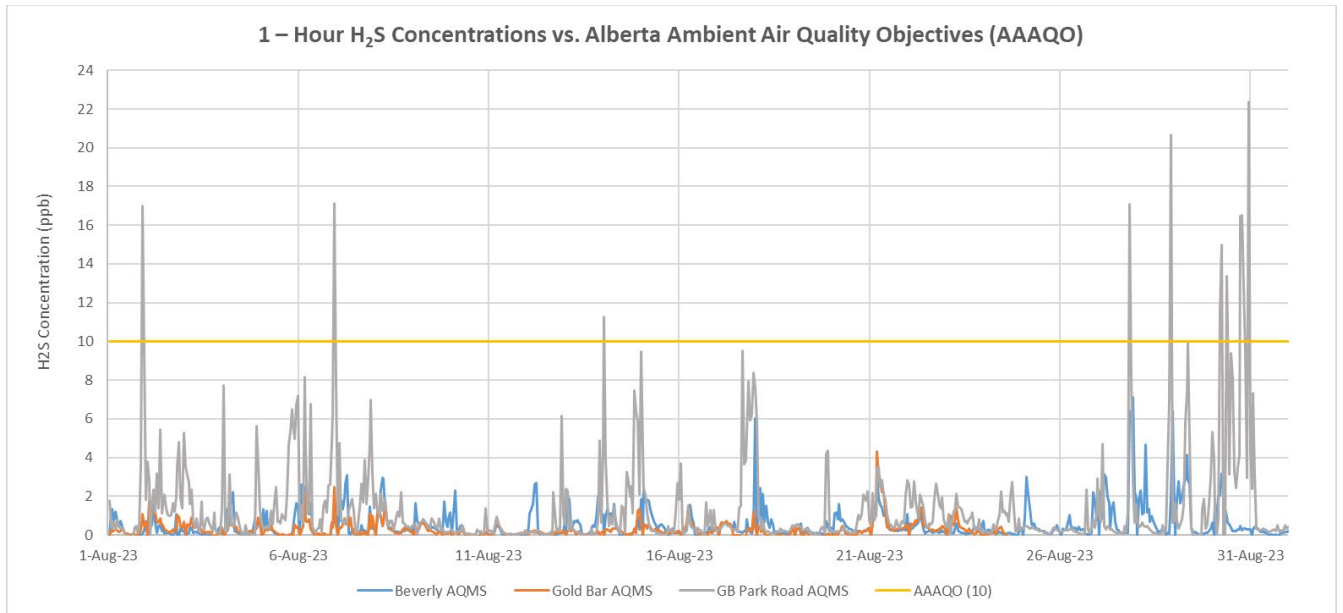
Figure 2: 1-Hour H 2 S Concentrations vs. Alberta Ambient Air Quality Objectives (AAAQO 10)
