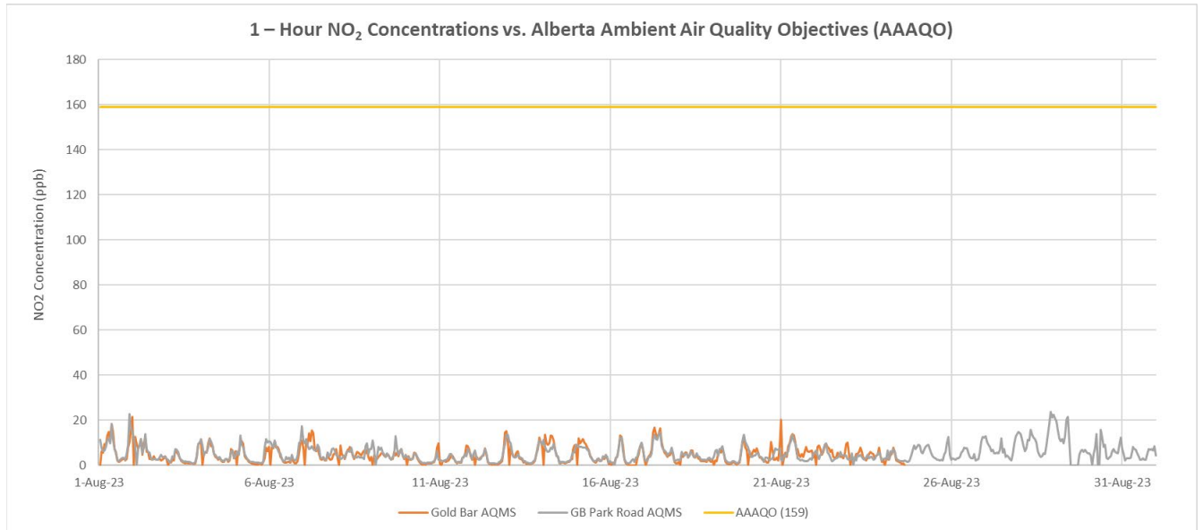
Figure 6: 1-Hour NO 2 Concentrations vs. Alberta Ambient Air Quality Objectives (AAAQO 159)
