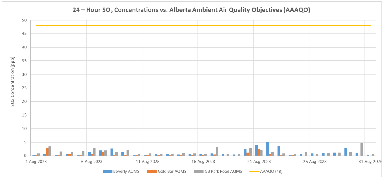
Figure 5: 24-Hour SO 2 Concentrations vs. Alberta Ambient Air Quality Objectives (AAAQO 48)
