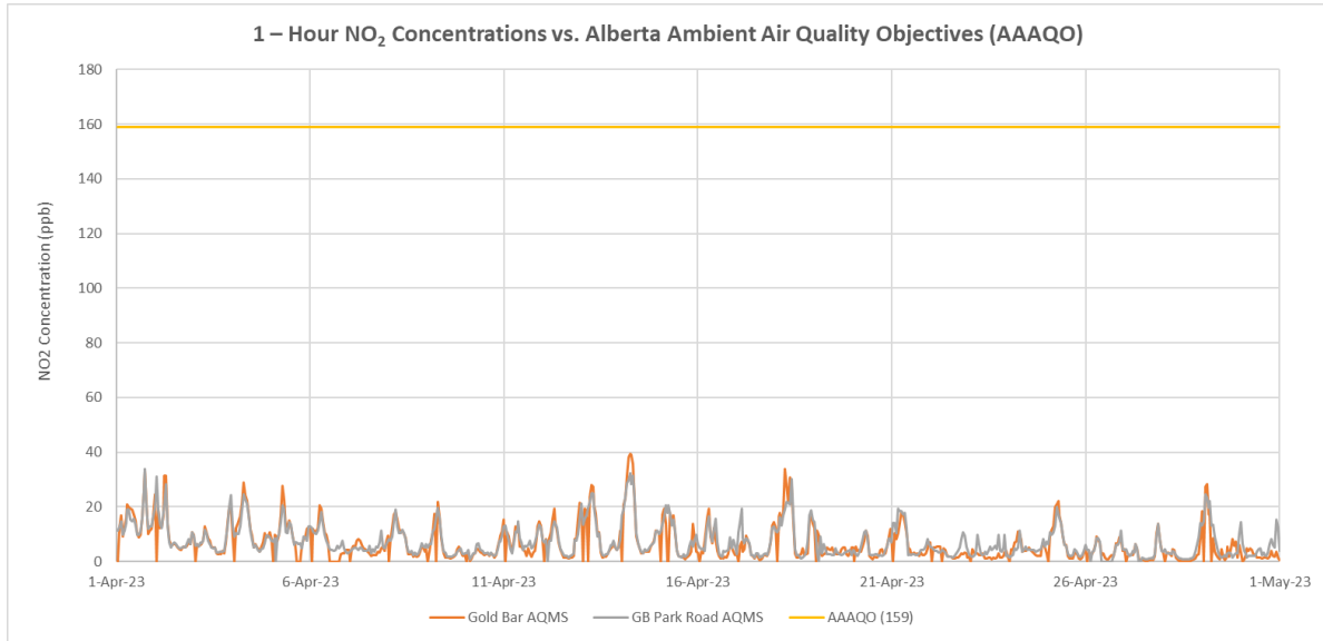
Figure 6: 1-Hour NO 2 Concentrations vs. Alberta Ambient Air Quality Objectives (AAAQO 159)
